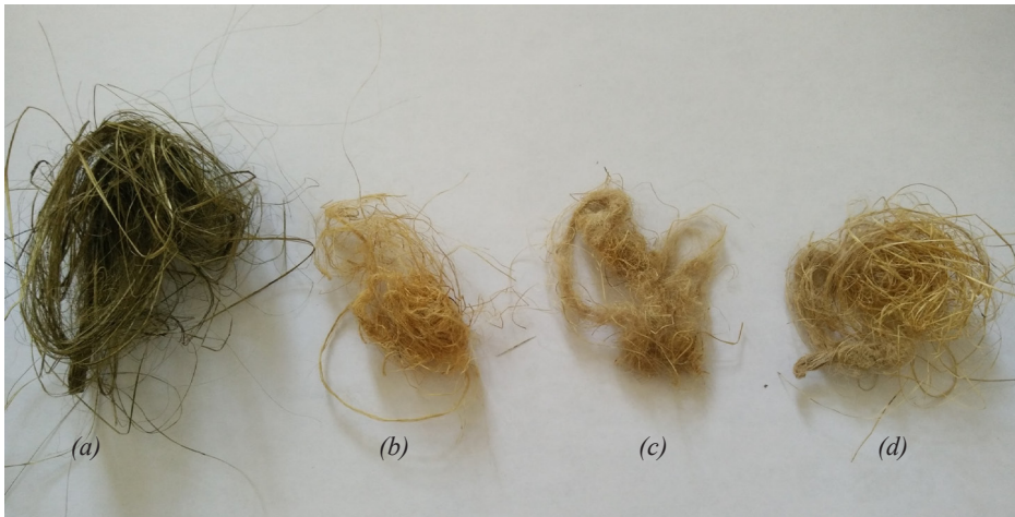
Figure 2. Pictures of a) The pristine LeLeF and LeLeF treated with b) 6 wt% NaOH, c) 8 wt% NaOH and d) 10 wt% NaOH
